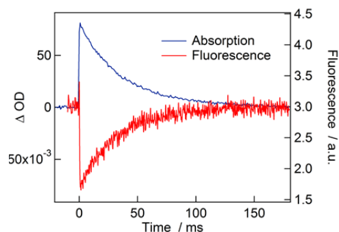
Fig. 1 Fluorescence switching with fast photochromism.
