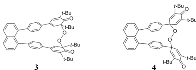
Figure 2. The molecular structures of two peroxide-bridged O 2 adducts ( 3 and 4 ).
